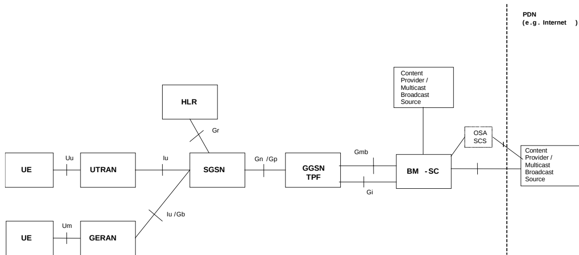
Figure 9: Configuration of MBMS entities
