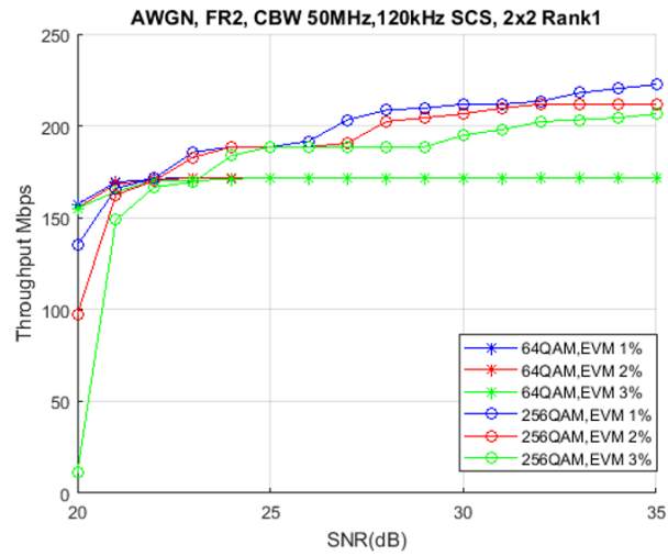
Figure 5.2.1.5-3: simulation results (Option d PN model)
