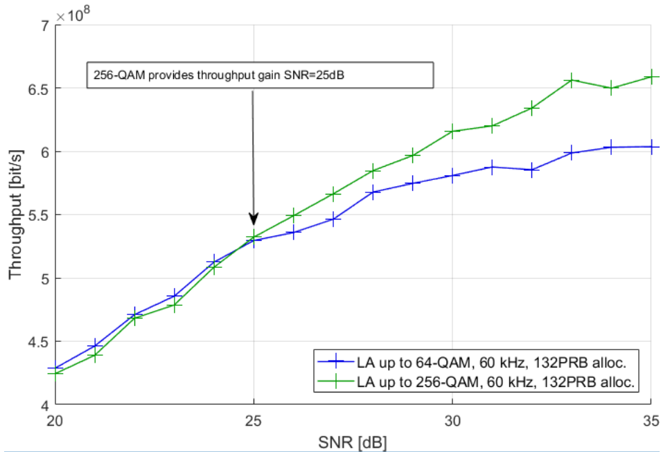
Figure 5.2.1.3-5: Throughput for rank-2 transmissions with 2% EVM for Tx and Rx excluding EVM from phase noise
