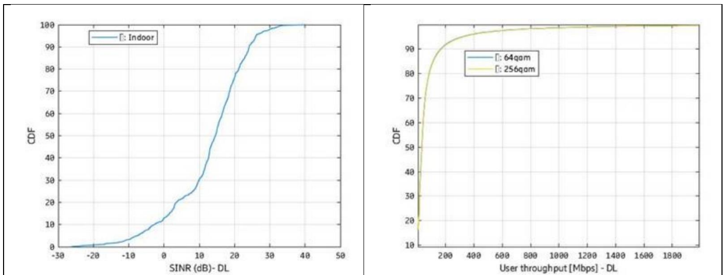
Figure 5.2.2.4-2: System-level indoor base station scenario SINR distribution and average user throughput
