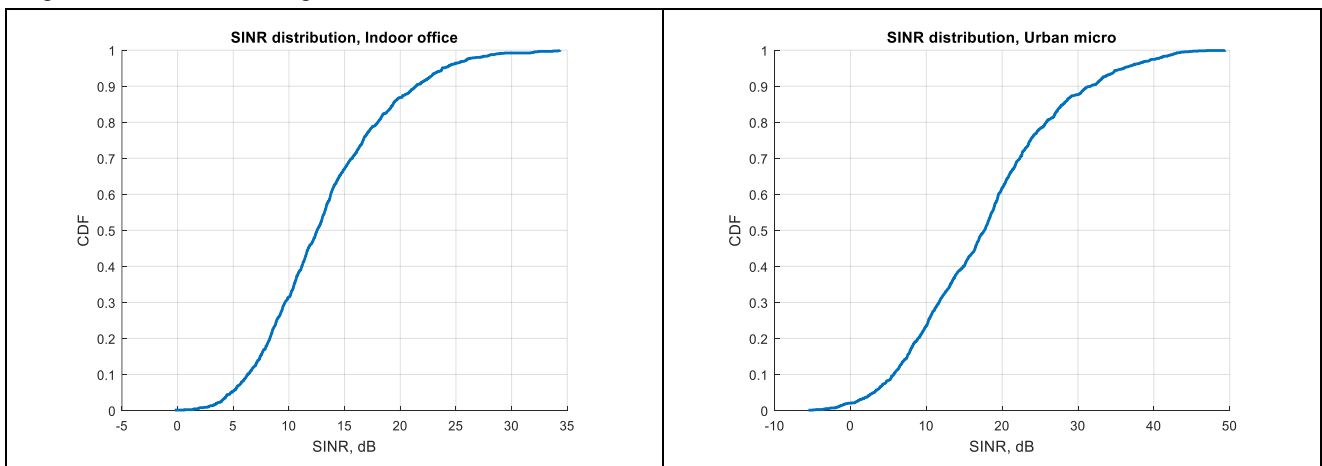
Figure 5.2.2.3-1: System-level large scale SINR distribution
