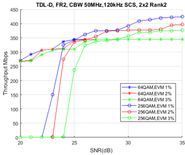
Figure 5.2.1.5-2: simulation results (Option a PN model)
