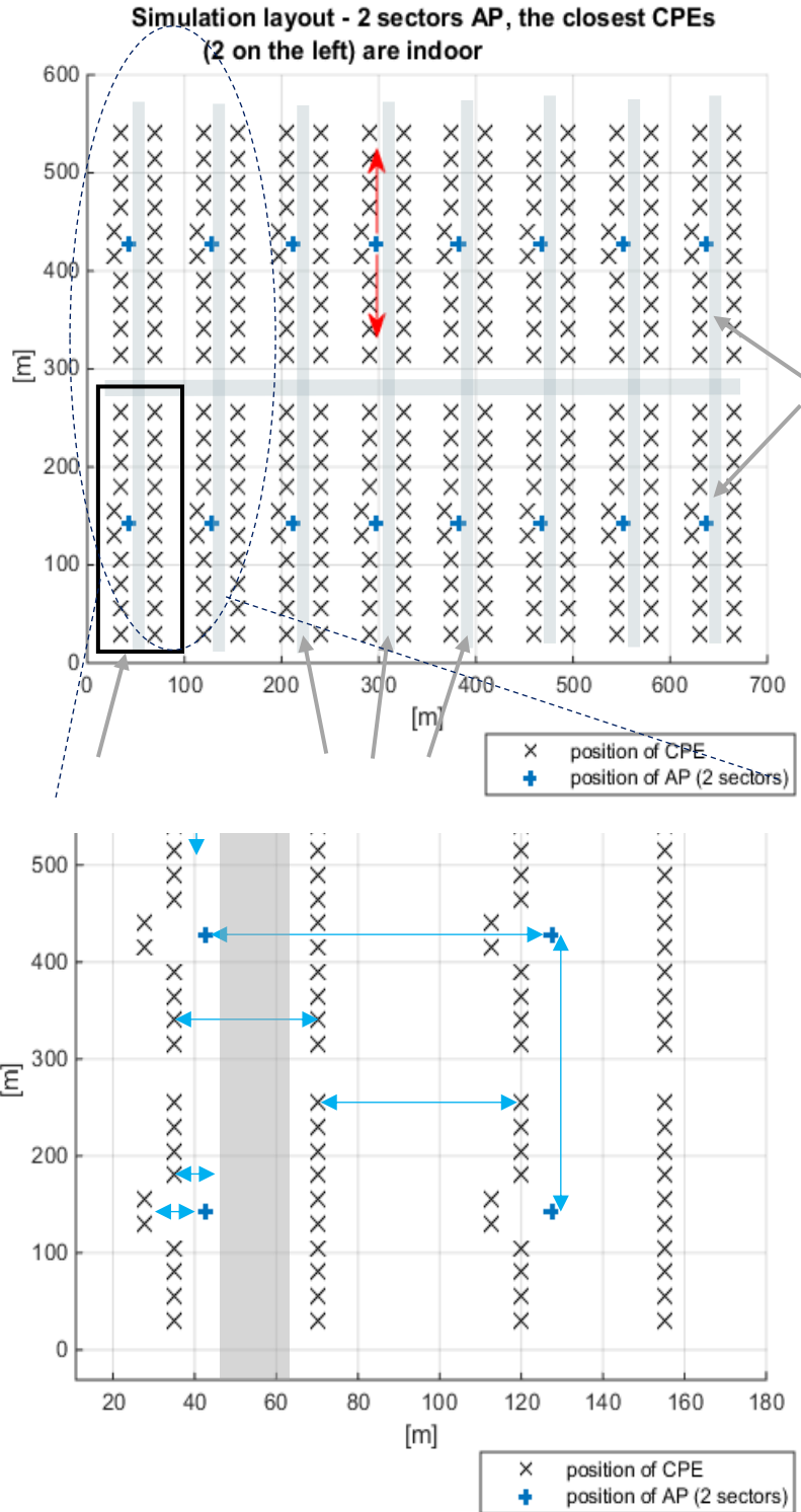
Figure A.2-1: Simulation layout
