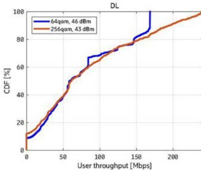
Figure 5.2.2.4-1: User throughput considering simple traffic assumptions
