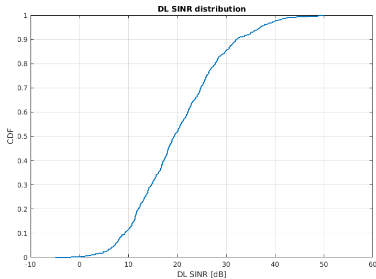
Figure 5.2.2.5-1: System level simulation results
