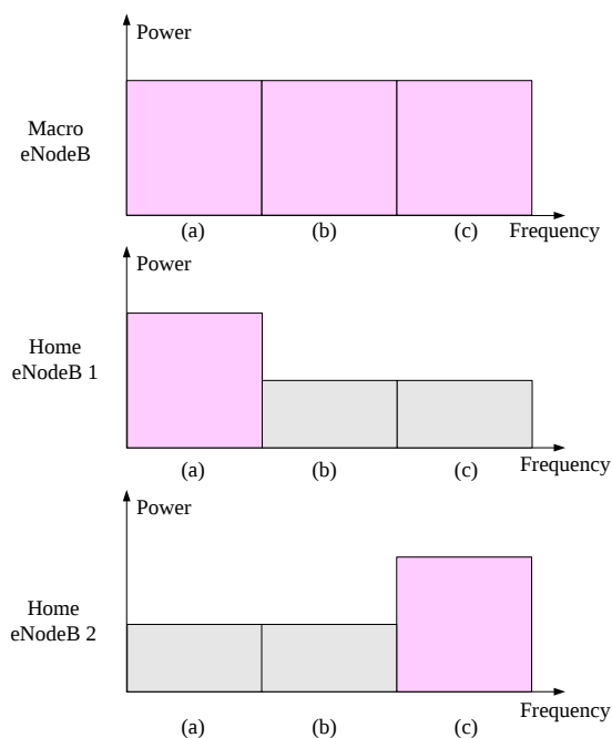
Figure 5.1-1 Frequency Partitioning
